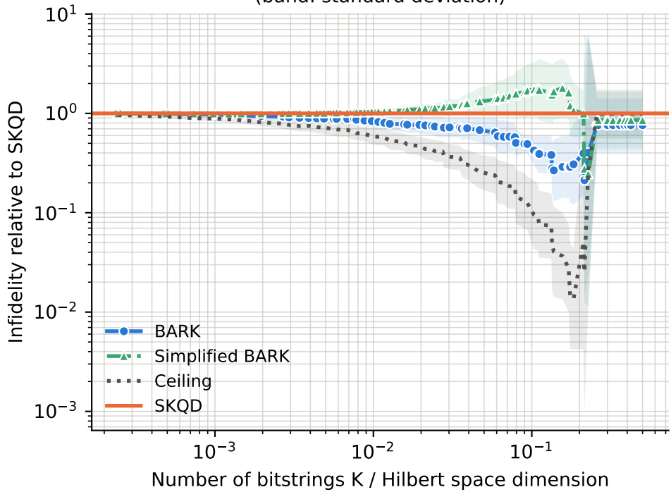
runs per point -- BARK: 11-20, Ceiling: 11-20, SKQD: 11-20, Simplified BARK: 11-20
