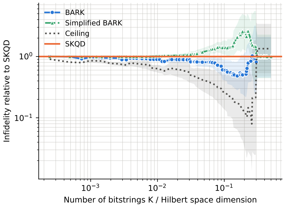
runs per point -- BARK: 4-41, Ceiling: 4-41, SKQD: 4-41, Simplified BARK: 4-41
