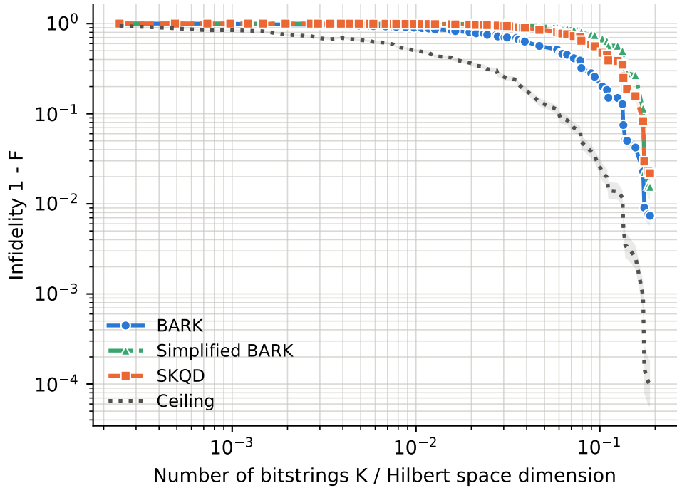
runs per point -- BARK: 18-55, Ceiling: 18-55, SKQD: 18-55, Simplified BARK: 18-55
