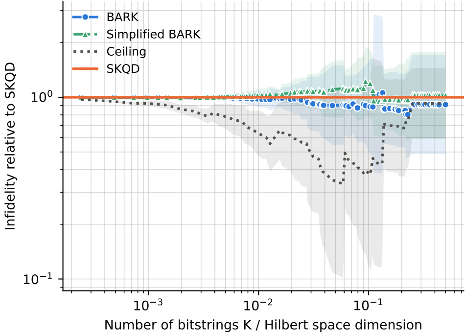
runs per point -- BARK: 14-85, Ceiling: 14-85, SKQD: 14-85, Simplified BARK: 14-85
