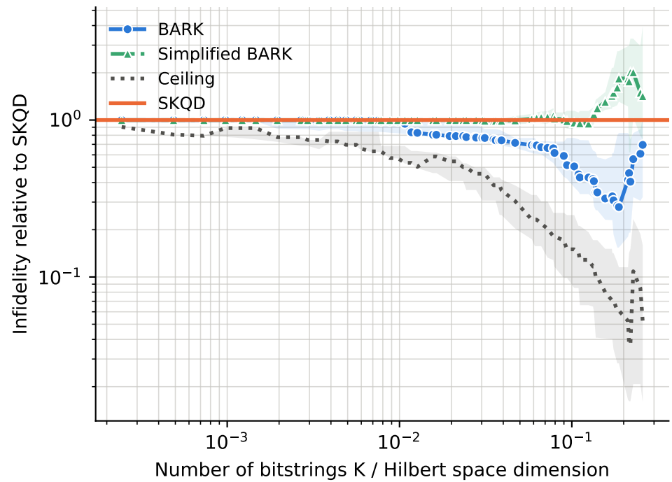
runs per point -- BARK: 6-44, Ceiling: 6-44, SKQD: 6-44, Simplified BARK: 6-44
