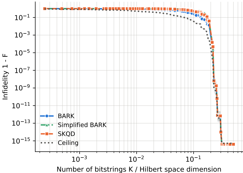
runs per point -- BARK: 30-101, Ceiling: 30-101, SKQD: 30-101, Simplified BARK: 30-101
