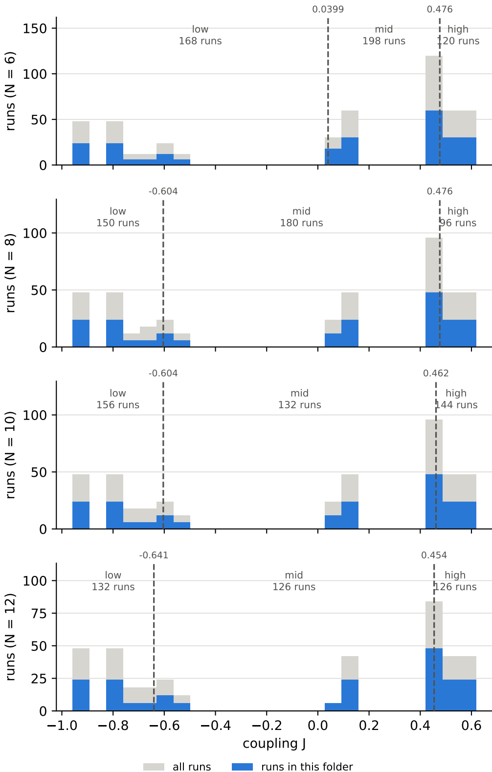
coupling J over all runs, and the cuts behind the bins lattice dimension = 1
