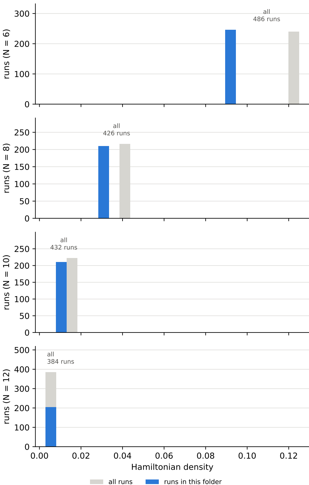
Hamiltonian density over all runs, and the cuts behind the bins lattice dimension = 1
