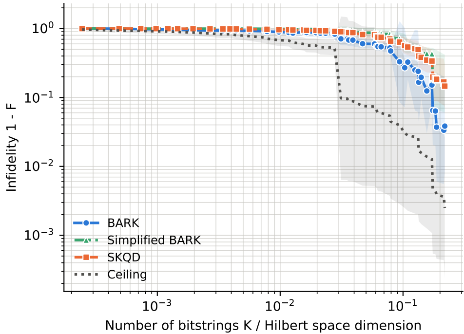
runs per point -- BARK: 30-60, Ceiling: 30-60, SKQD: 30-60, Simplified BARK: 30-60
