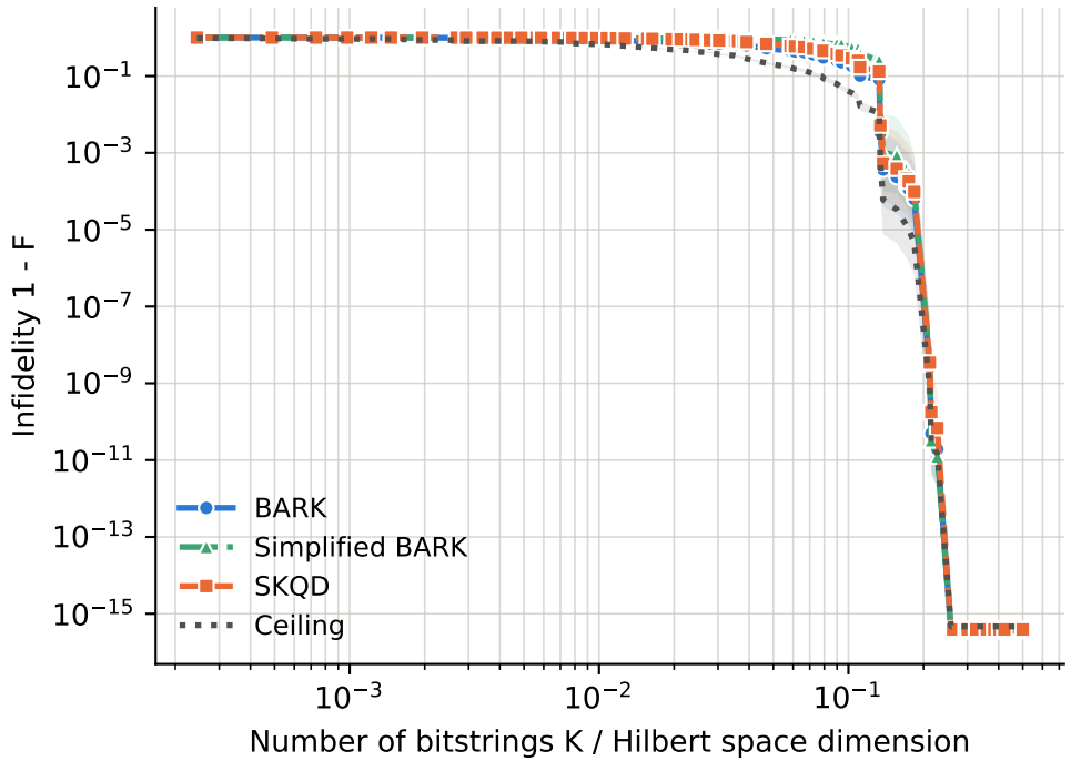
runs per point -- BARK: 4-30, Ceiling: 4-30, SKQD: 4-30, Simplified BARK: 4-30
