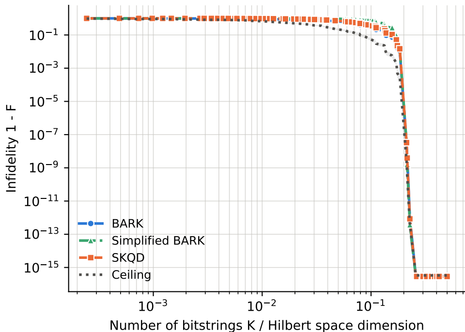
runs per point -- BARK: 8-29, Ceiling: 8-29, SKQD: 8-29, Simplified BARK: 8-29
