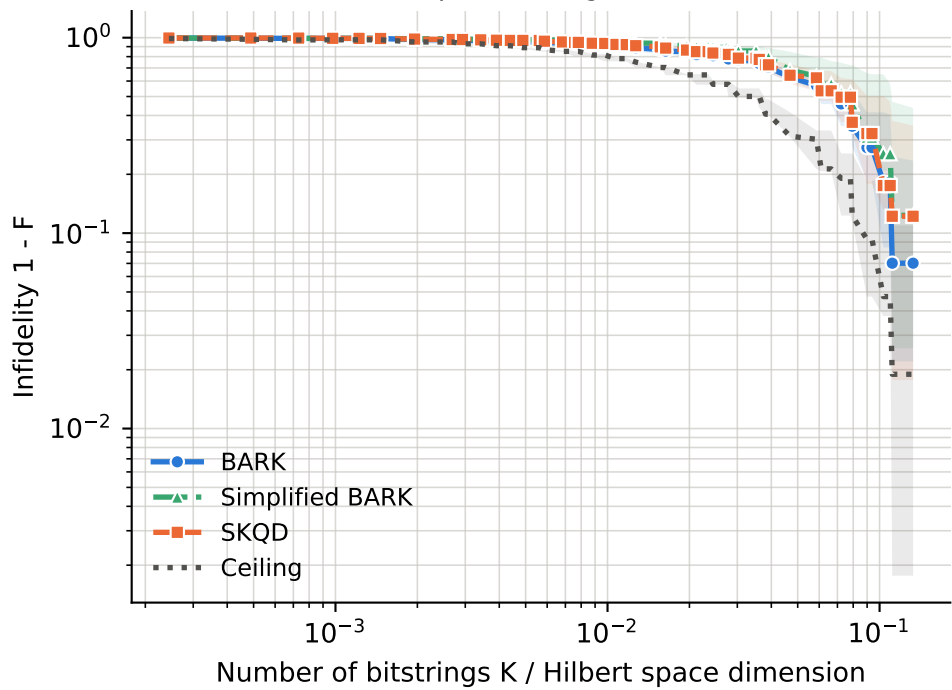
runs per point -- BARK: 7-28, Ceiling: 7-28, SKQD: 7-28, Simplified BARK: 7-28
