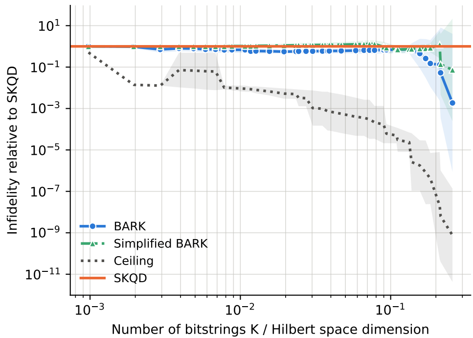
runs per point -- BARK: 16-31, Ceiling: 16-31, SKQD: 16-31, Simplified BARK: 16-31
