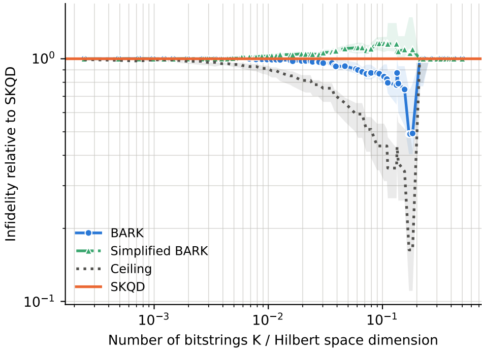
runs per point -- BARK: 4-16, Ceiling: 4-16, SKQD: 4-16, Simplified BARK: 4-16
