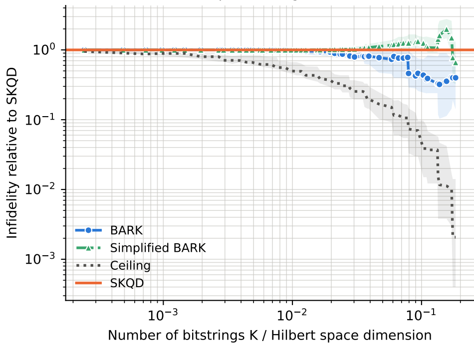
runs per point -- BARK: 14-28, Ceiling: 14-28, SKQD: 14-28, Simplified BARK: 14-28
