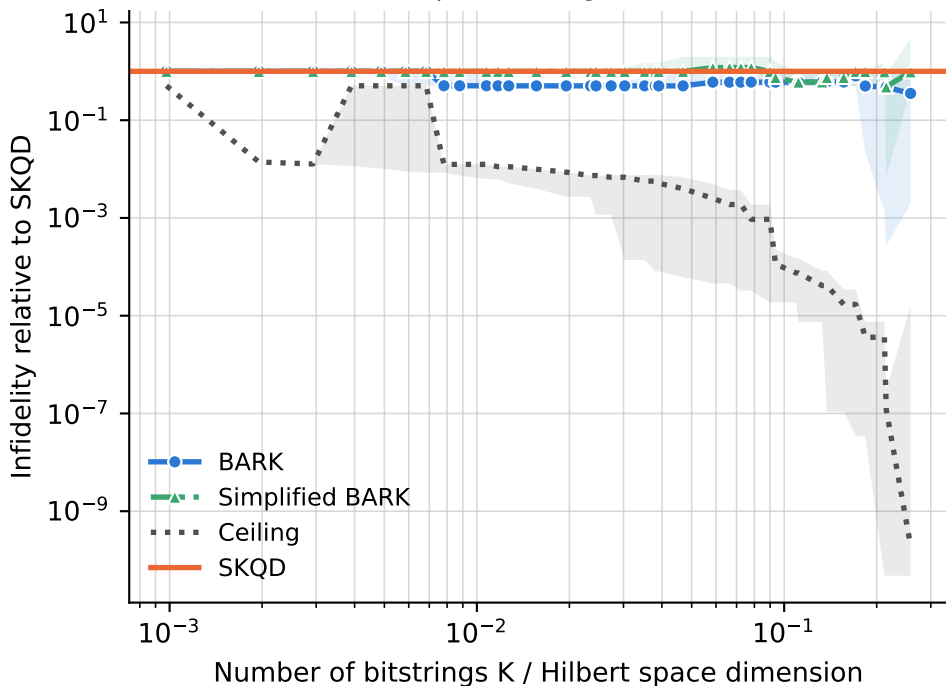
runs per point -- BARK: 11-23, Ceiling: 11-23, SKQD: 11-23, Simplified BARK: 11-23
