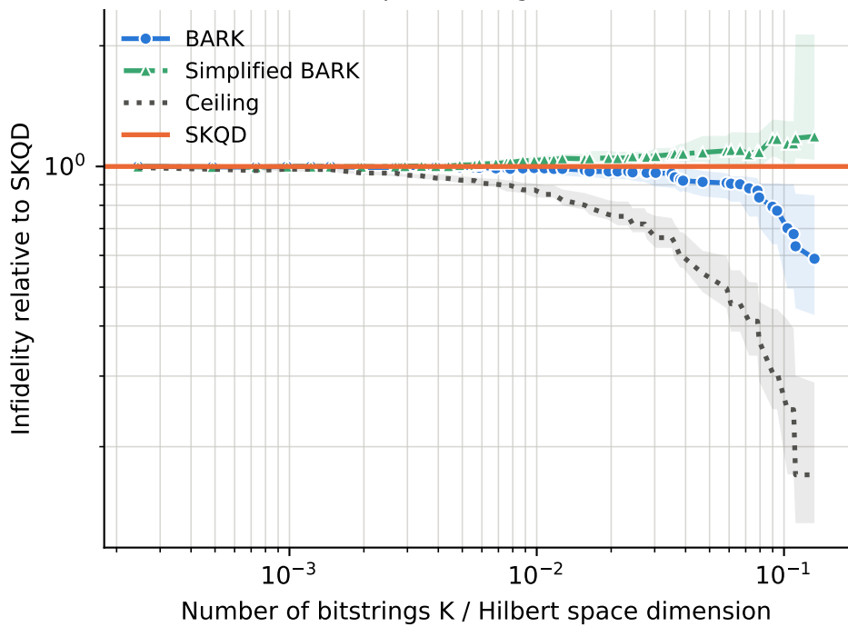
runs per point -- BARK: 20-52, Ceiling: 20-52, SKQD: 20-52, Simplified BARK: 20-52
