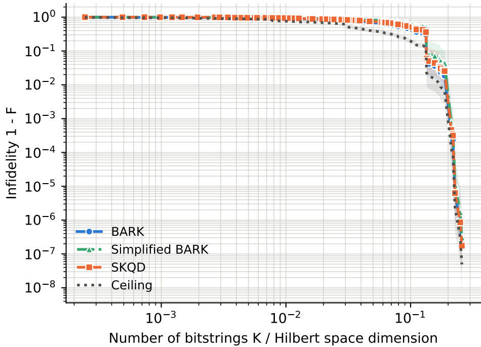
runs per point -- BARK: 13-79, Ceiling: 13-79, SKQD: 13-79, Simplified BARK: 13-79
