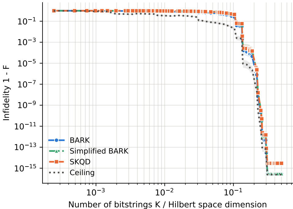
runs per point -- BARK: 54-234, Ceiling: 54-234, SKQD: 54-234, Simplified BARK: 54-234
