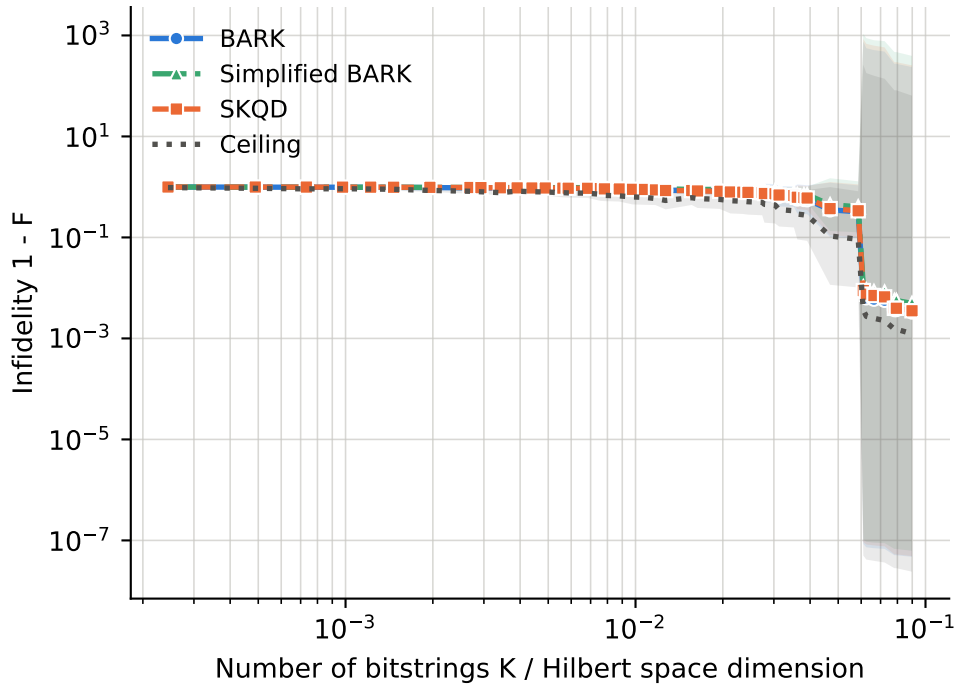
runs per point -- BARK: 6-54, Ceiling: 6-54, SKQD: 6-54, Simplified BARK: 6-54
