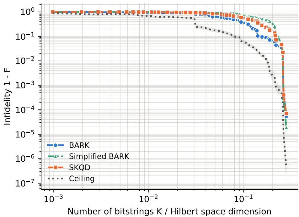
runs per point -- BARK: 6-48, Ceiling: 6-48, SKQD: 6-48, Simplified BARK: 6-48
