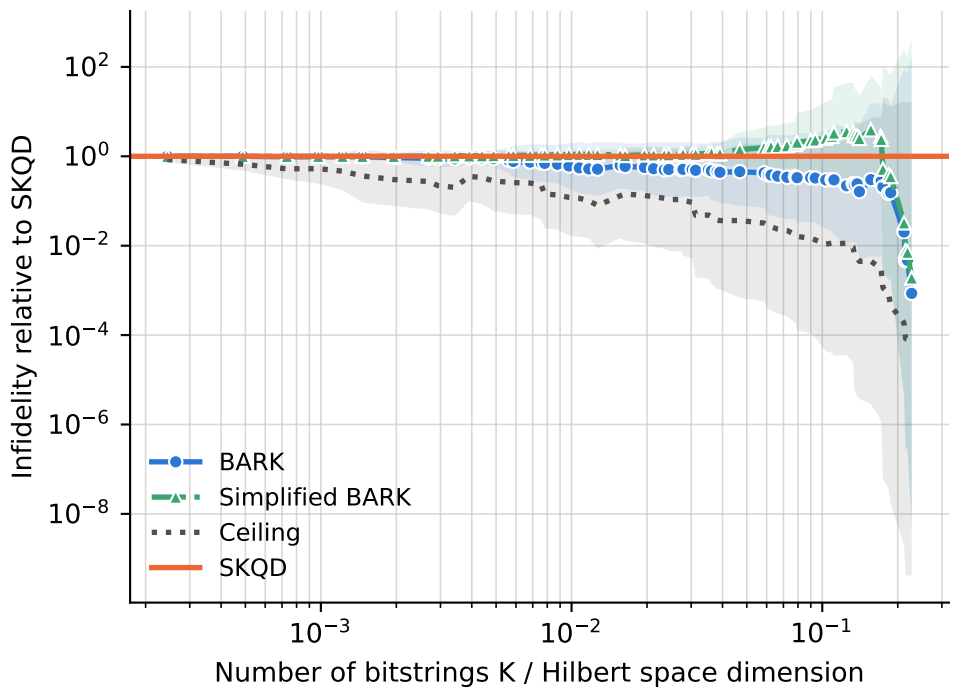
runs per point -- BARK: 12-72, Ceiling: 12-72, SKQD: 12-72, Simplified BARK: 12-72
