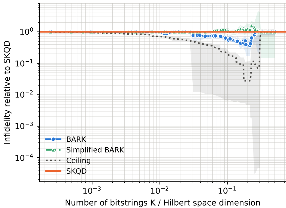
runs per point -- BARK: 6-30, Ceiling: 6-30, SKQD: 6-30, Simplified BARK: 6-30
