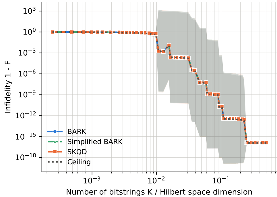
runs per point -- BARK: 12-54, Ceiling: 12-54, SKQD: 12-54, Simplified BARK: 12-54
