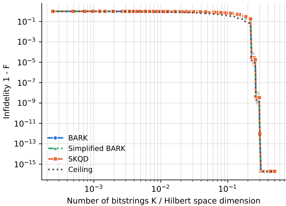
runs per point -- BARK: 36-144, Ceiling: 36-144, SKQD: 36-144, Simplified BARK: 36-144
