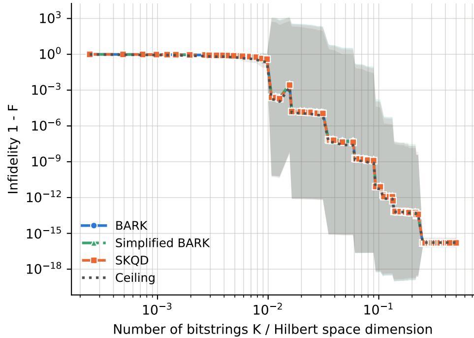
runs per point -- BARK: 11-41, Ceiling: 11-41, SKQD: 11-41, Simplified BARK: 11-41
