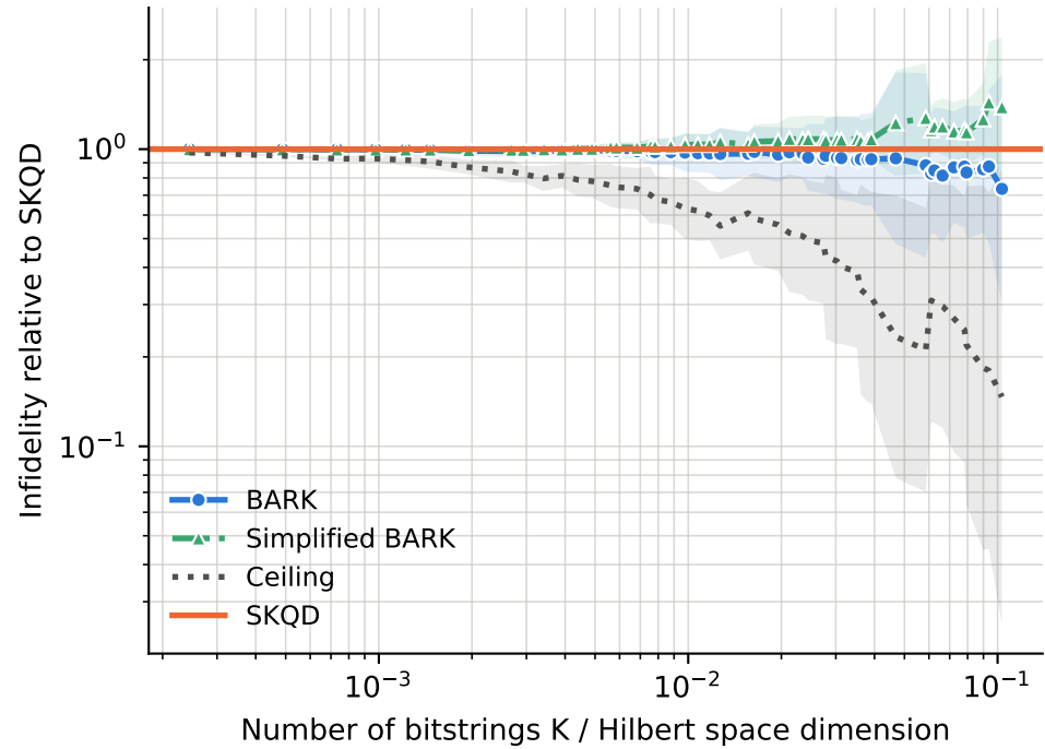
runs per point -- BARK: 4-15, Ceiling: 4-15, SKQD: 4-15, Simplified BARK: 4-15
