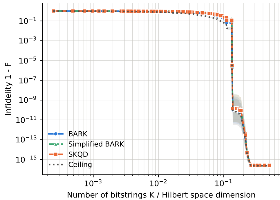
runs per point -- BARK: 13-30, Ceiling: 13-30, SKQD: 13-30, Simplified BARK: 13-30
