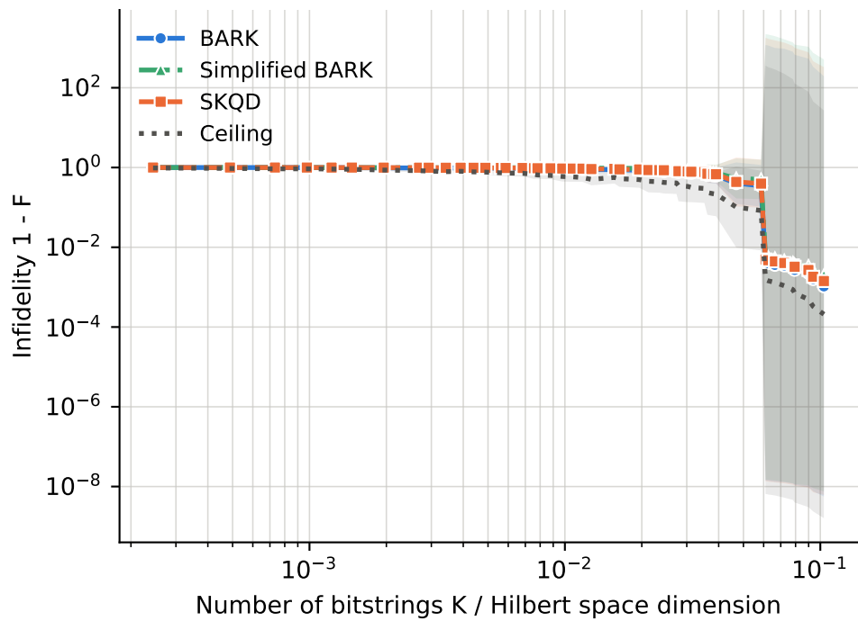
runs per point -- BARK: 4-15, Ceiling: 4-15, SKQD: 4-15, Simplified BARK: 4-15
