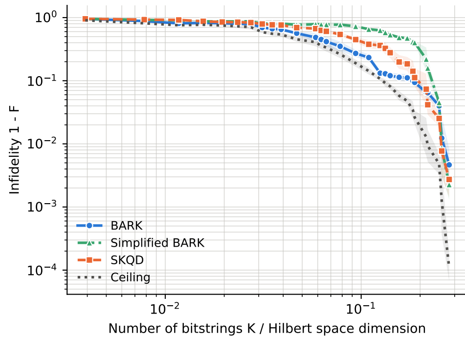
runs per point -- BARK: 2-6, Ceiling: 2-6, SKQD: 2-6, Simplified BARK: 2-6
