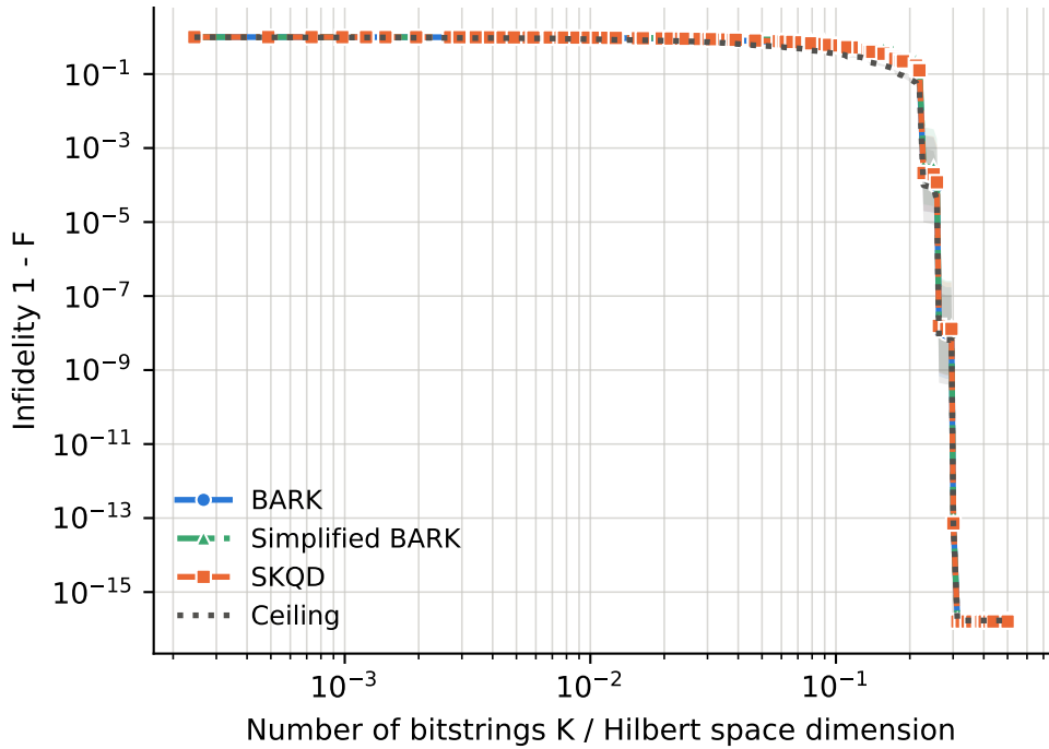
runs per point -- BARK: 6-33, Ceiling: 6-33, SKQD: 6-33, Simplified BARK: 6-33
