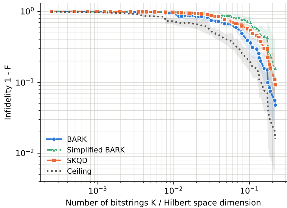
runs per point -- BARK: 3-13, Ceiling: 3-13, SKQD: 3-13, Simplified BARK: 3-13
