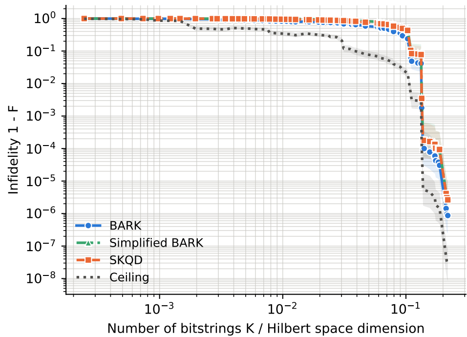
runs per point -- BARK: 36-138, Ceiling: 36-138, SKQD: 36-138, Simplified BARK: 36-138
