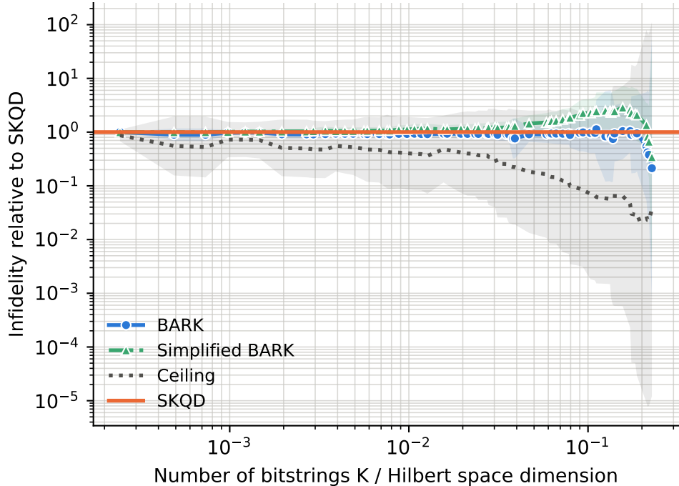
runs per point -- BARK: 6-39, Ceiling: 6-39, SKQD: 6-39, Simplified BARK: 6-39
