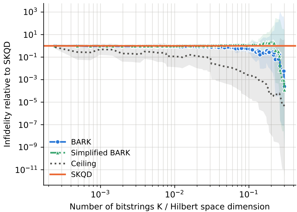
runs per point -- BARK: 13-96, Ceiling: 13-96, SKQD: 13-96, Simplified BARK: 13-96
