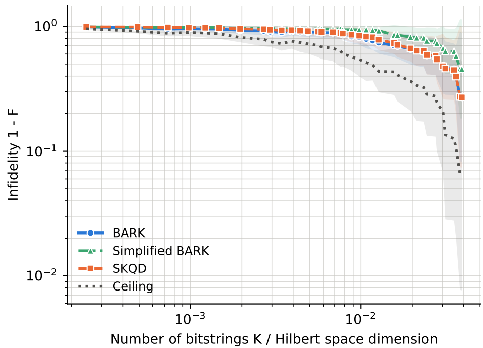
runs per point -- BARK: 6-30, Ceiling: 6-30, SKQD: 6-30, Simplified BARK: 6-30
