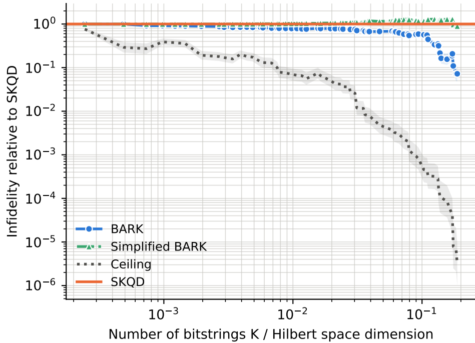
runs per point -- BARK: 30-79, Ceiling: 30-79, SKQD: 30-79, Simplified BARK: 30-79
