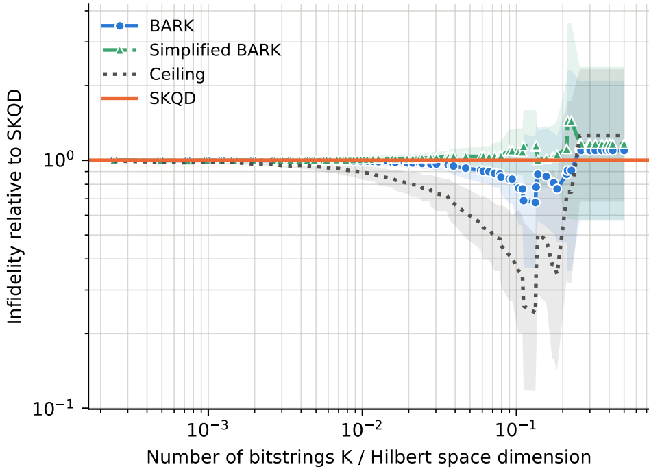
runs per point -- BARK: 12-60, Ceiling: 12-60, SKQD: 12-60, Simplified BARK: 12-60
