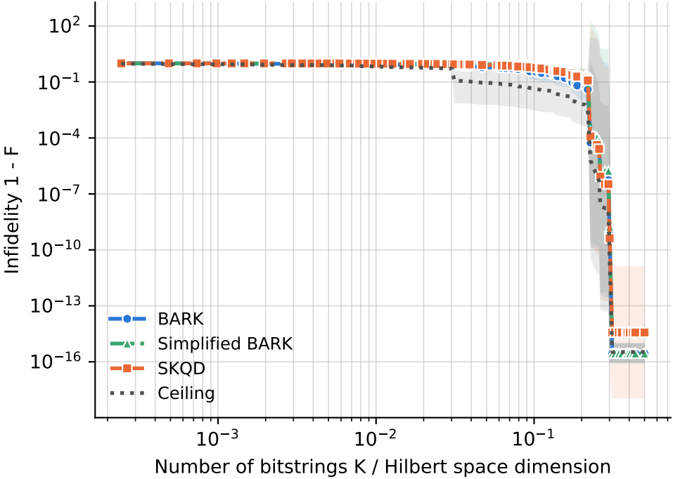
runs per point -- BARK: 36-168, Ceiling: 36-168, SKQD: 36-168, Simplified BARK: 36-168
