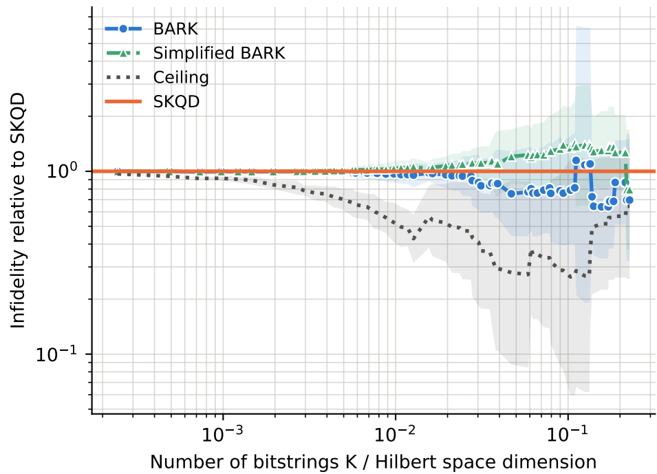
runs per point -- BARK: 7-38, Ceiling: 7-38, SKQD: 7-38, Simplified BARK: 7-38
