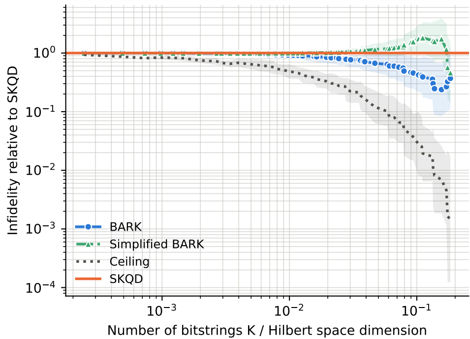
runs per point -- BARK: 13-40, Ceiling: 13-40, SKQD: 13-40, Simplified BARK: 13-40
