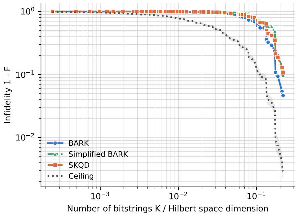
runs per point -- BARK: 16-33, Ceiling: 16-33, SKQD: 16-33, Simplified BARK: 16-33
