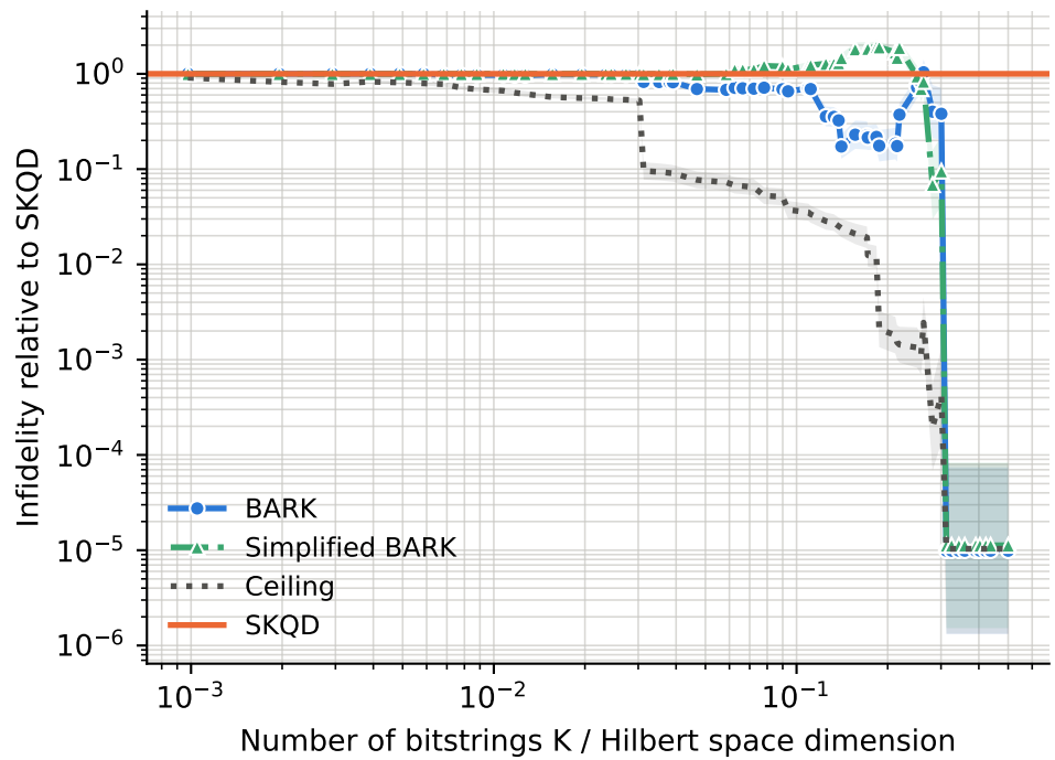
runs per point -- BARK: 3-39, Ceiling: 3-39, SKQD: 3-39, Simplified BARK: 3-39
