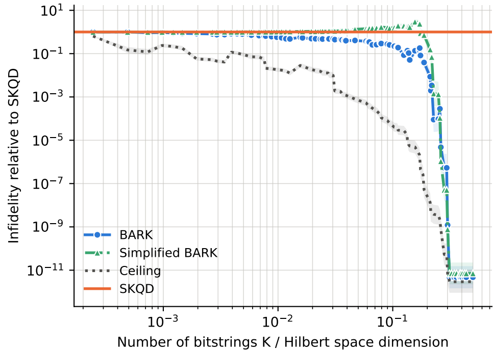
runs per point -- BARK: 19-100, Ceiling: 19-100, SKQD: 19-100, Simplified BARK: 19-100
