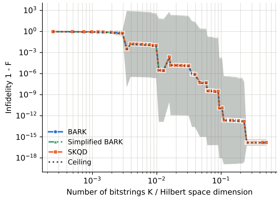
runs per point -- BARK: 18-79, Ceiling: 18-79, SKQD: 18-79, Simplified BARK: 18-79
