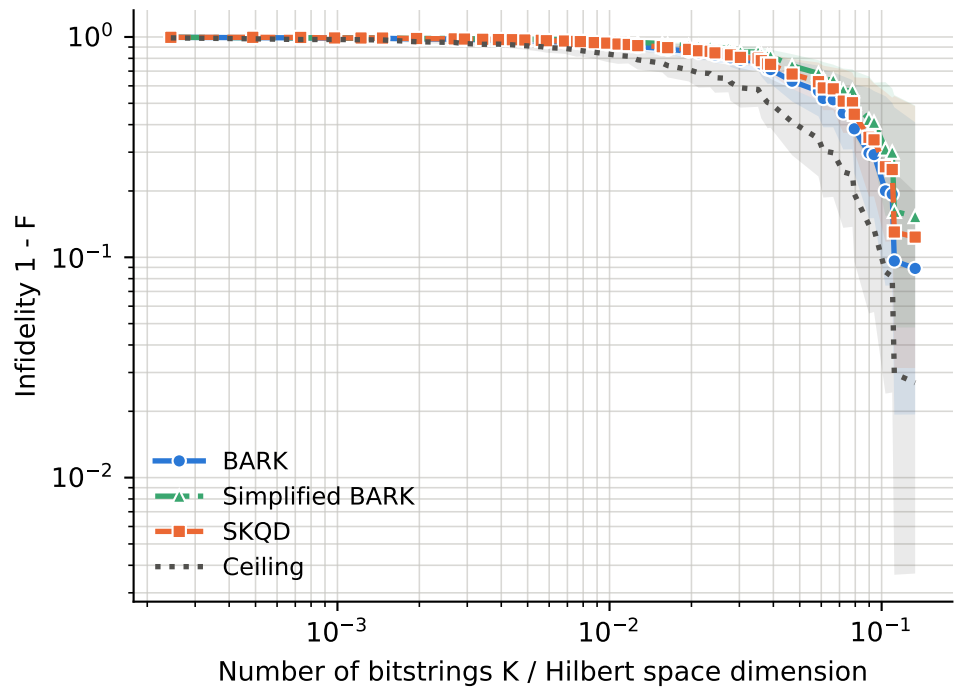
runs per point -- BARK: 7-25, Ceiling: 7-25, SKQD: 7-25, Simplified BARK: 7-25
