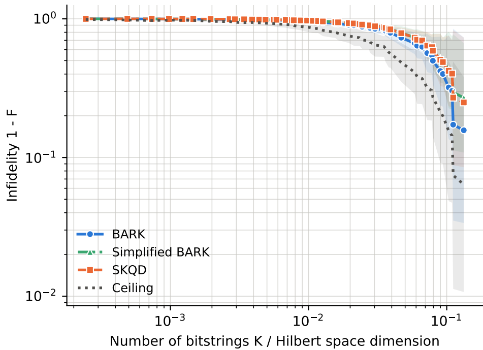
runs per point -- BARK: 5-32, Ceiling: 5-32, SKQD: 5-32, Simplified BARK: 5-32
