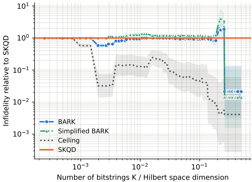
runs per point -- BARK: 1-15, Ceiling: 1-15, SKQD: 1-15, Simplified BARK: 1-15
