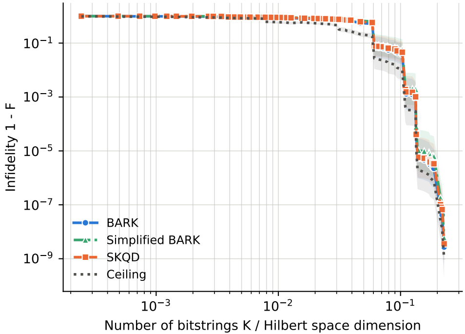
runs per point -- BARK: 21-88, Ceiling: 21-88, SKQD: 21-88, Simplified BARK: 21-88
