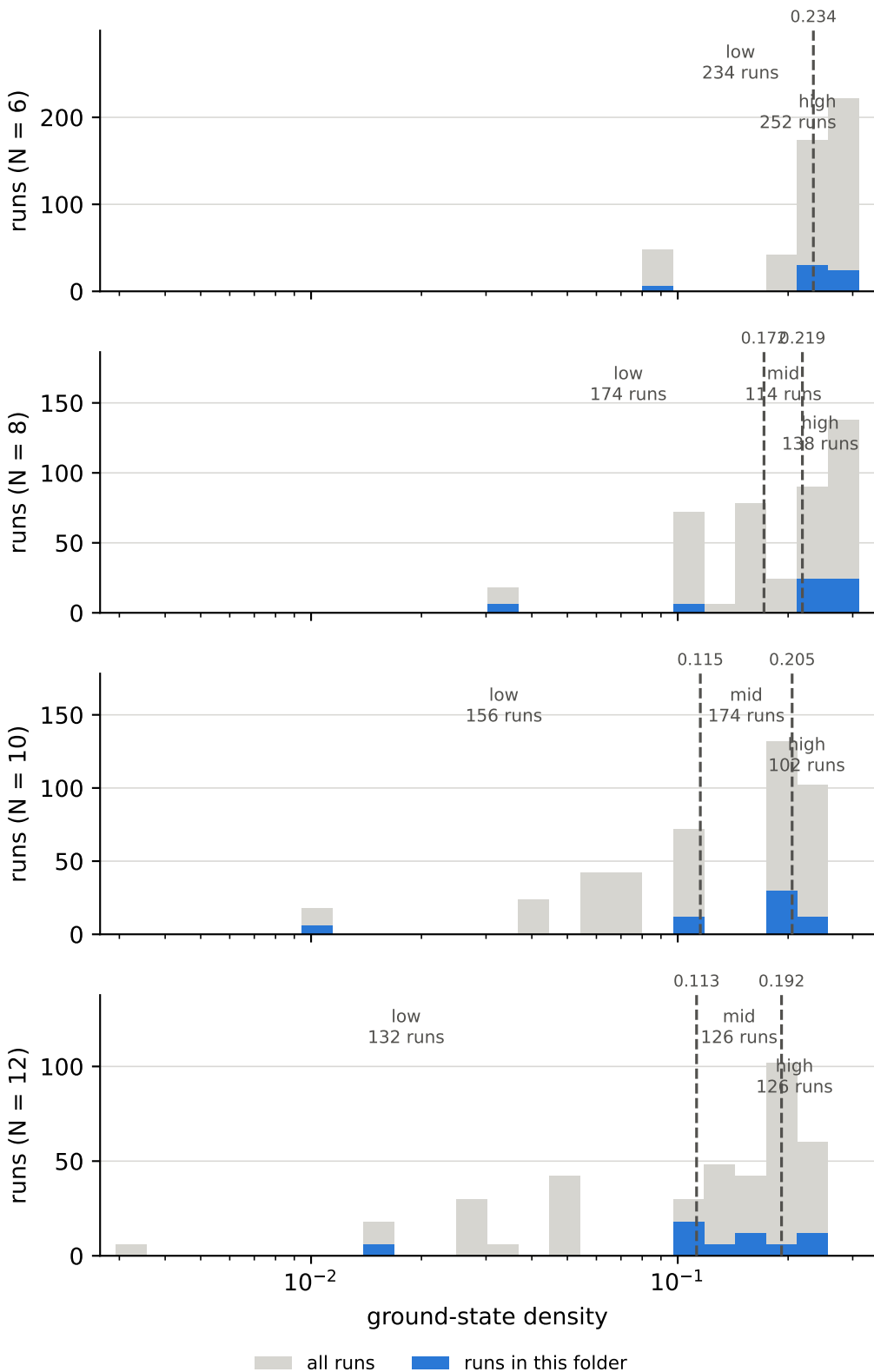
ground-state density over all runs, and the cuts behind the bins lattice dimension = 1, anisotropy delta = 0.5
